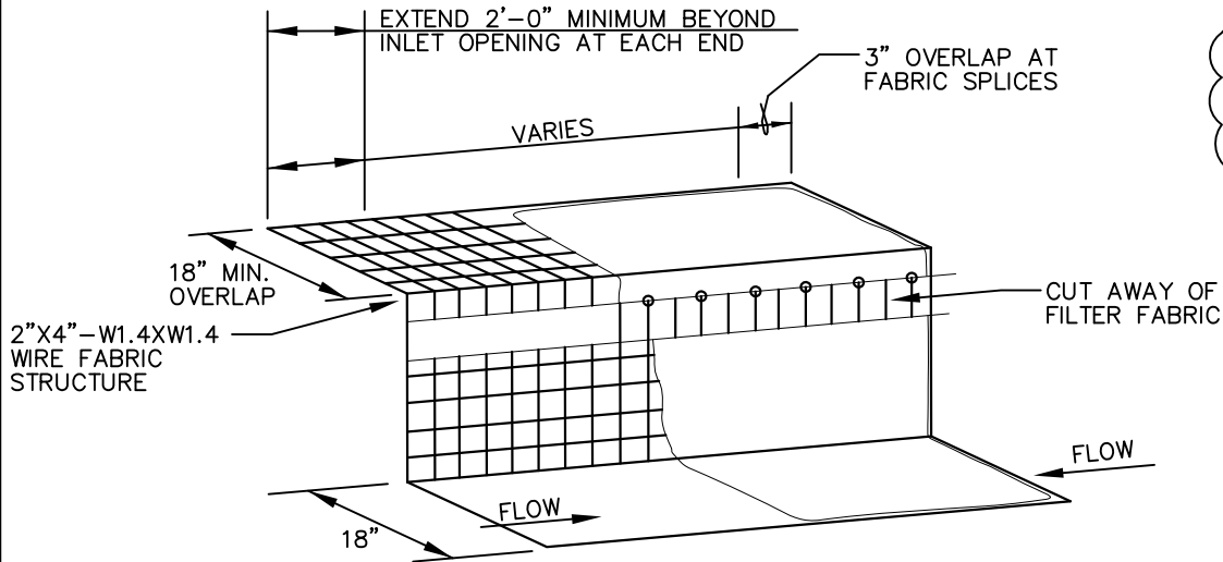
WIRE WEIR CURB INLET PROTECTION ISOMETRIC VIEW N.T.S.
