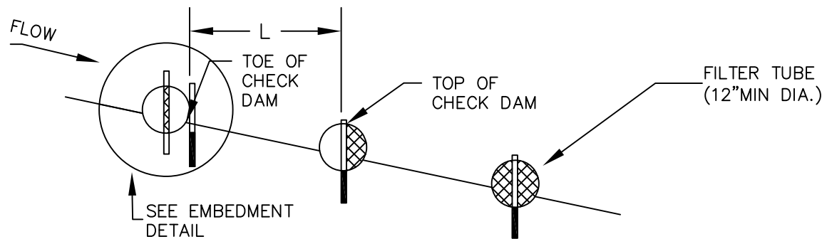
FILTER TUBE CHECK DAM PROFILE
