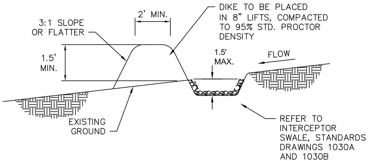
DIVERSION DIKE WITH SWALE CROSS SECTION N.T.S
