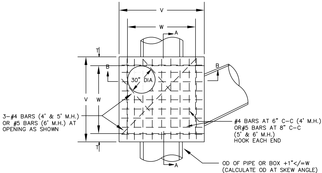
PLAN
