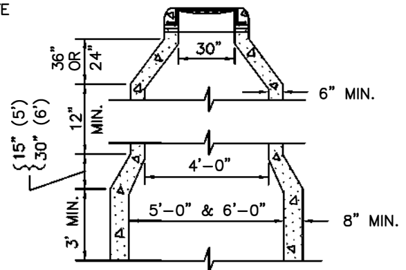
TRANSITION DETAIL FOR 5' & 6' DIA. M.H.'S
