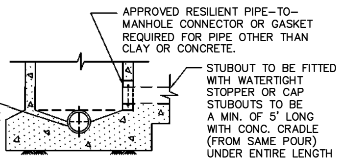
STUBOUT CONNECTION
