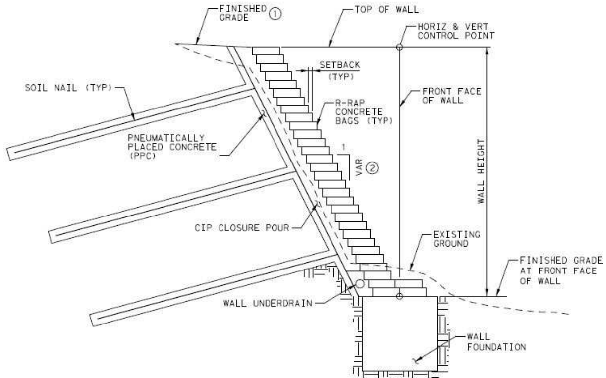
SOIL NAIL
