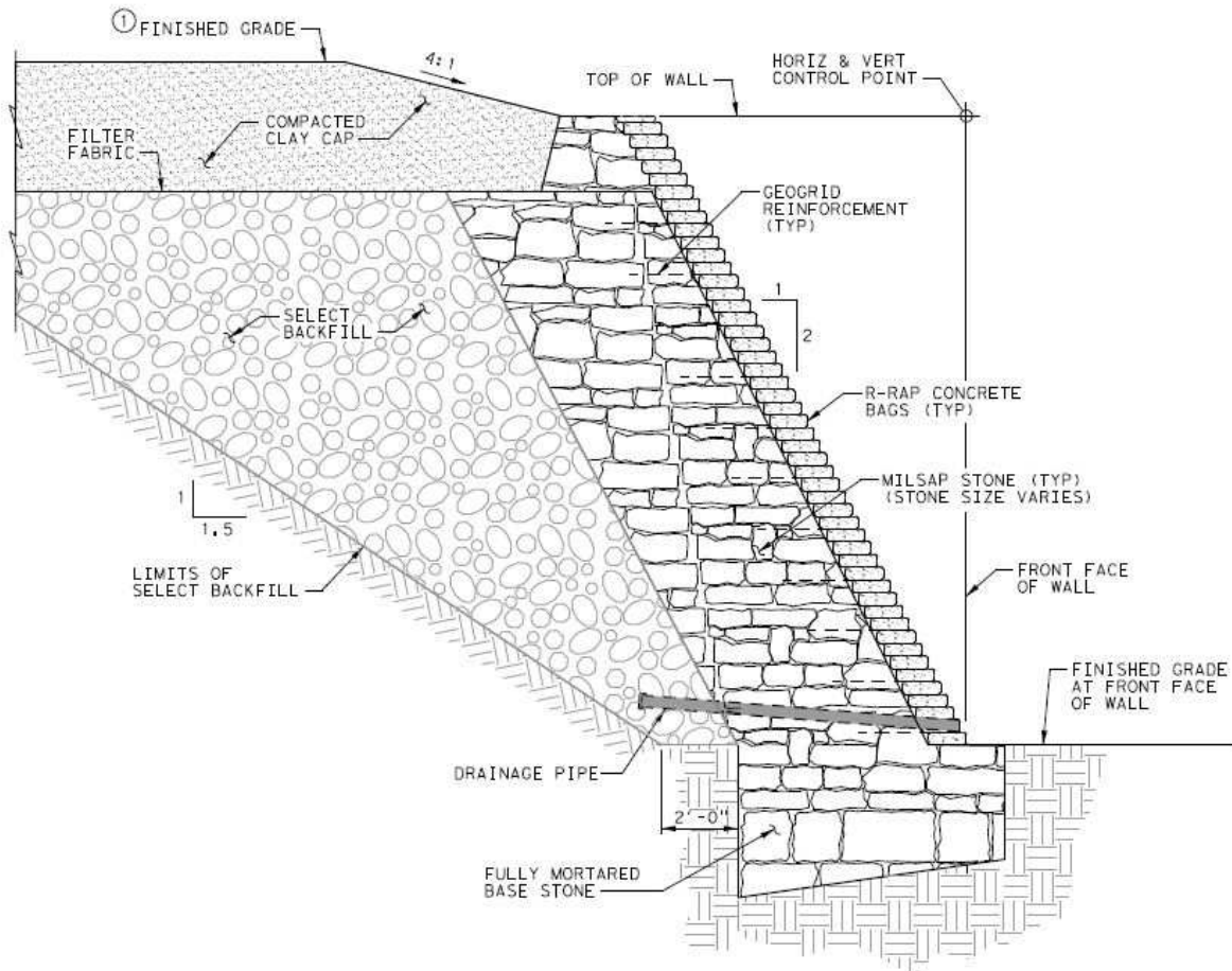
R-RAP AND MASONRY STONE
