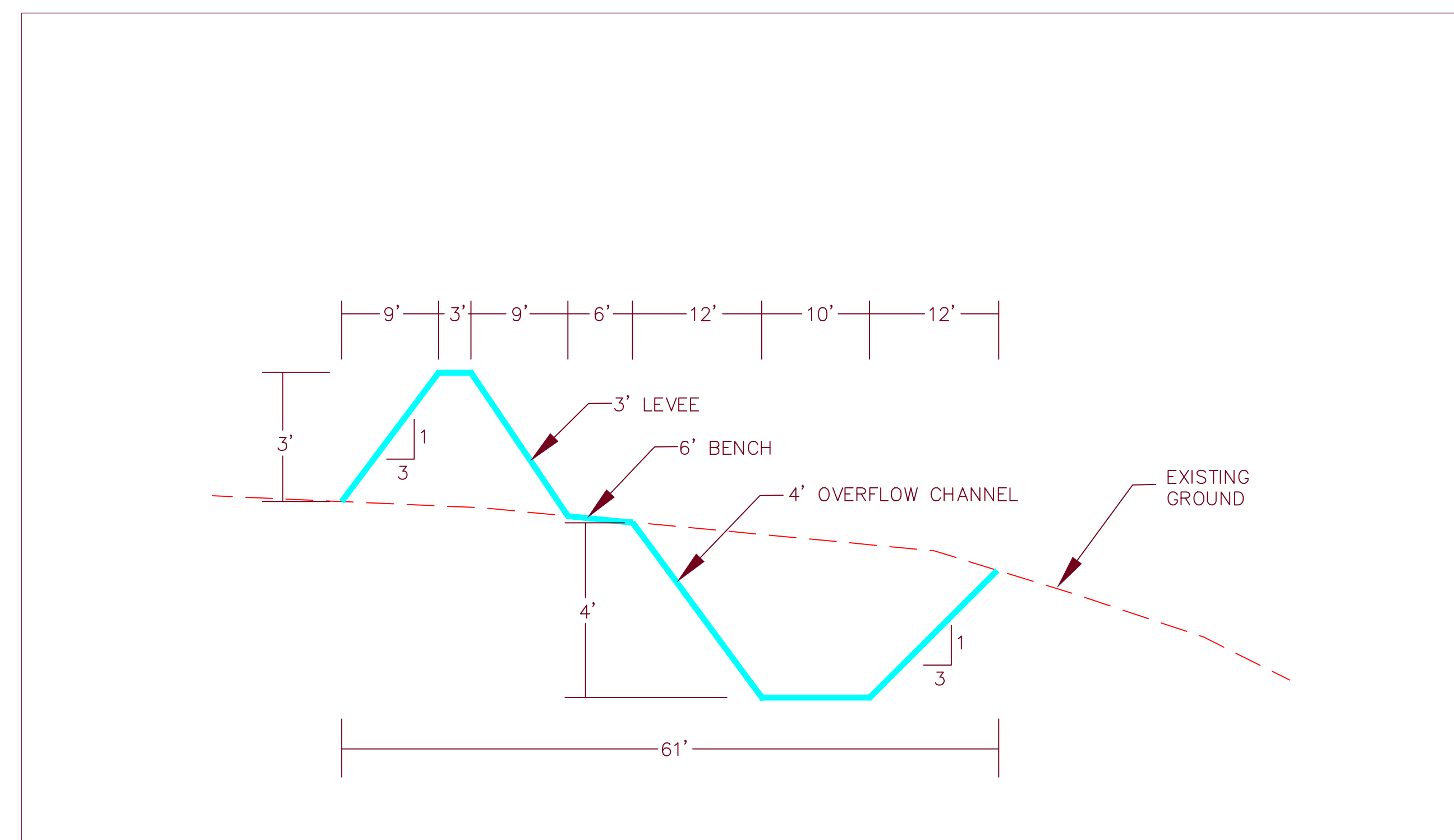
LEVEE AND OVERFLOW CHANNEL DETAIL SCALE: 1"=10' HOR; 1"=2.5' VER
