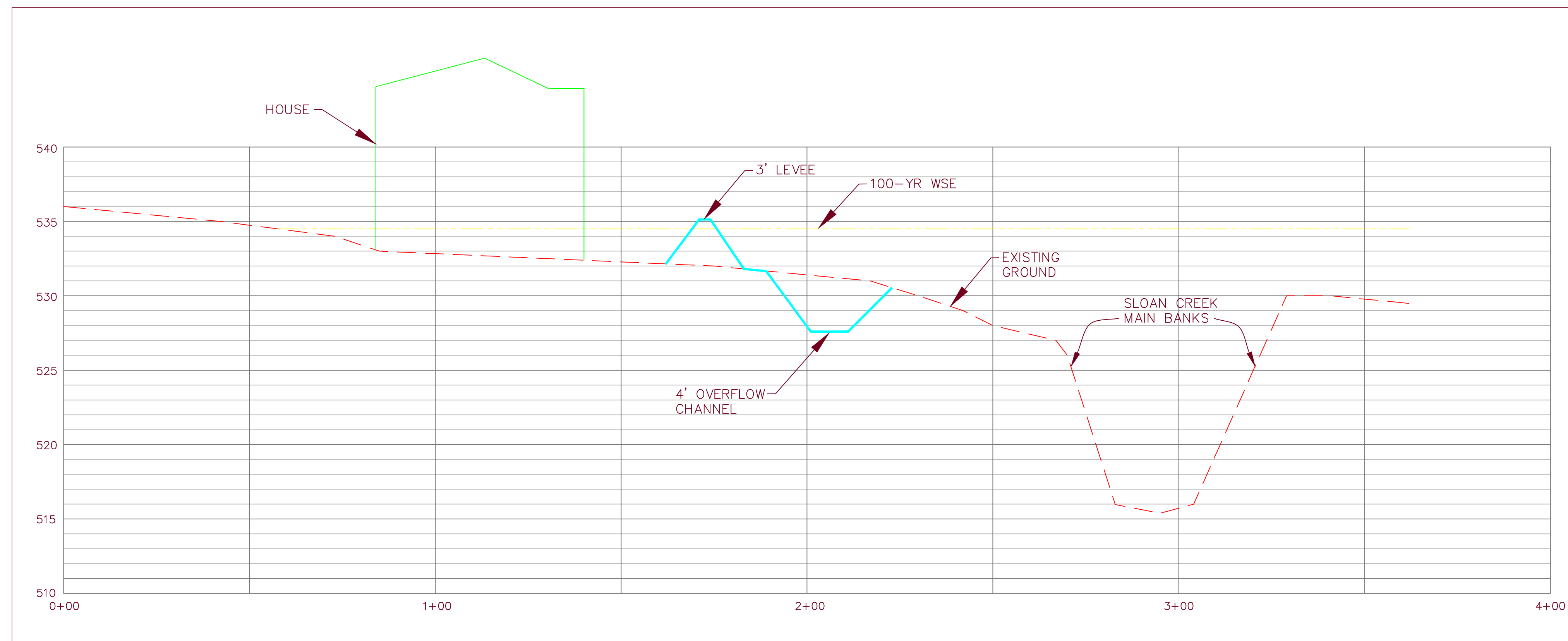
TYPICAL SECTION SCALE: 1"=20' HOR; 1"=5' VER
