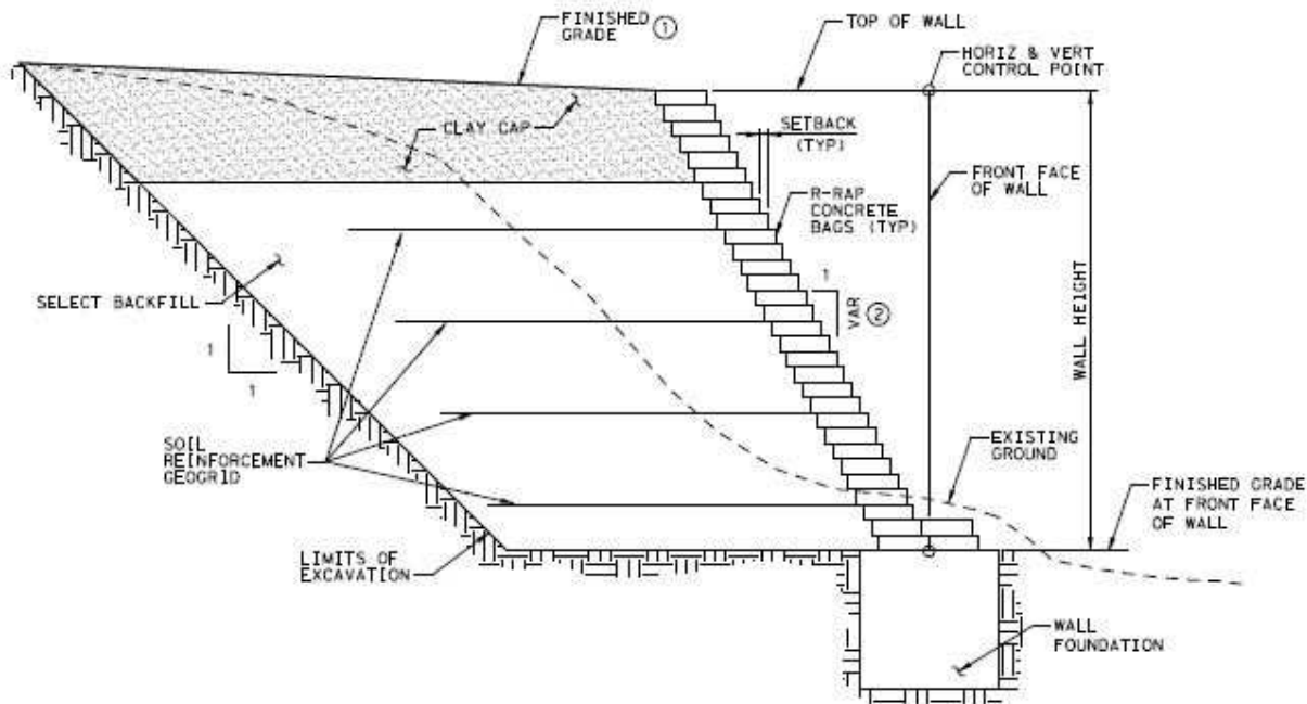
R-RAP AND GEOGRID
