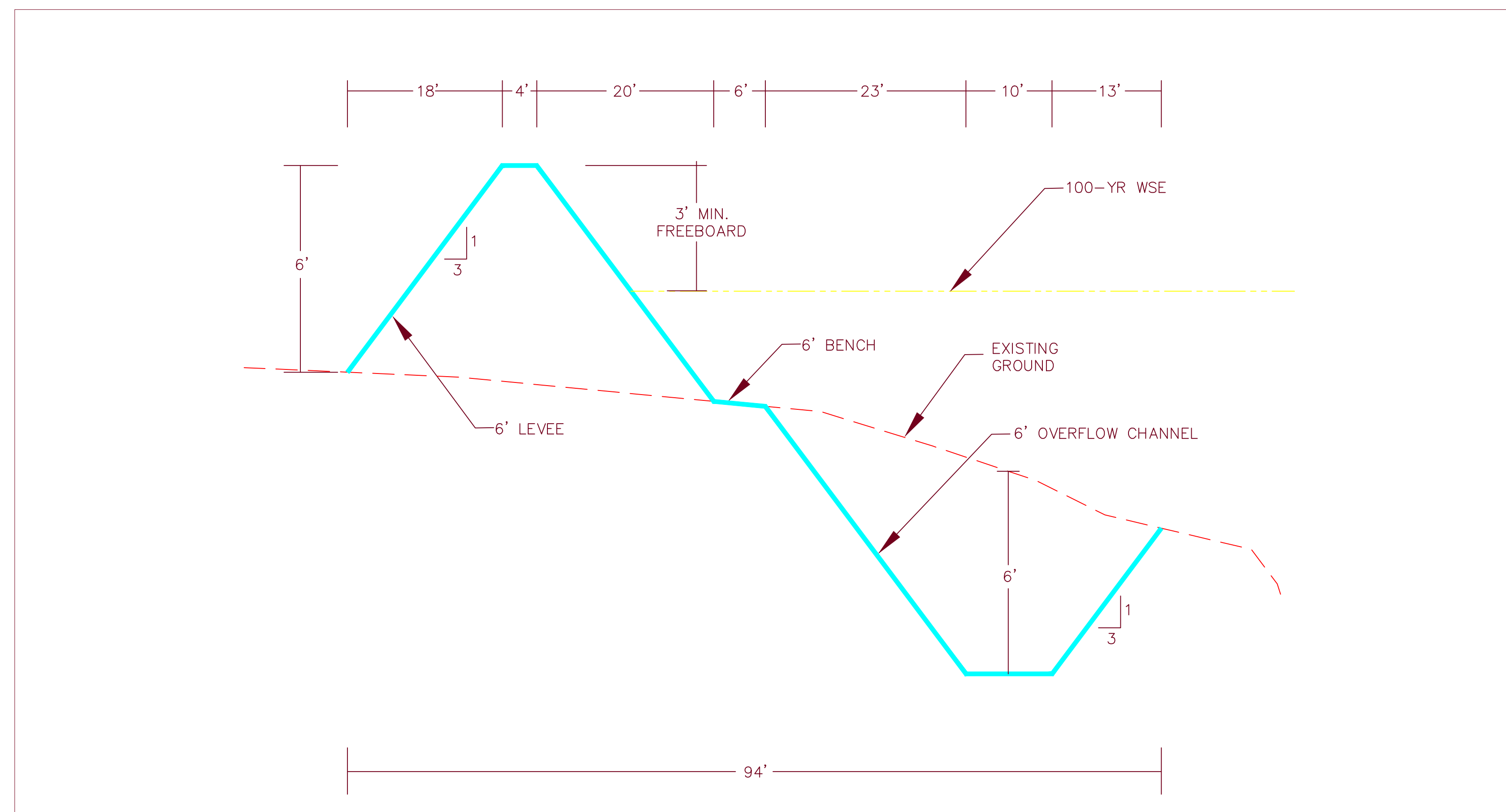
LEVEE AND OVERFLOW CHANNEL DETAIL SCALE: 1"=10' HOR; 1"=2.5' VER
