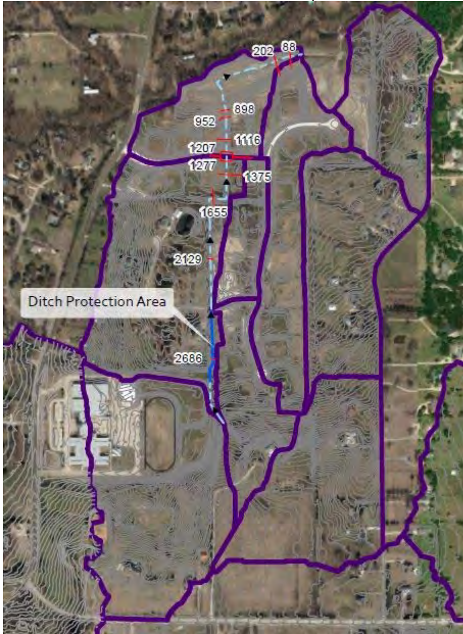
HEC-RAS Cross-sections and extents of ditch protection
